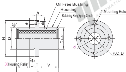
Round Flange OGJ02
