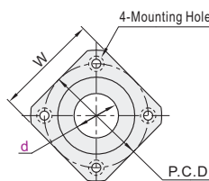
Square Flange OGJ32
