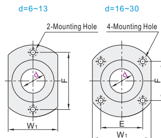
Compact Flange OGJ62
