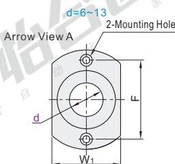
Compact Flange OGE62 OGF62
