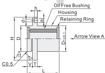
Round Flange OGE02 OGF02
