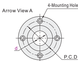
Round Flange OGE02 OGF02
