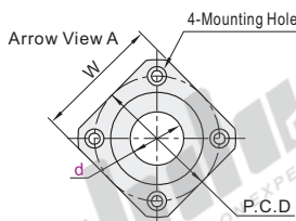
Square Flange OGE32 OGF32
