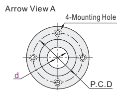
Round Flange OGB02
