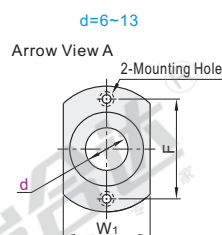
Compact Flange OGB62
