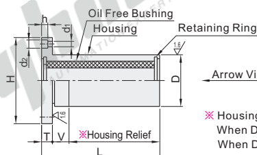
Square Flange OGB32
