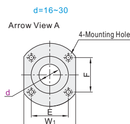
Compact Flange OGB62
