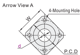
Square Flange OGB32
