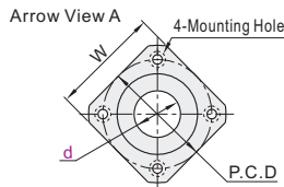
Square Flange OFZ86
