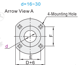
Compact Flange OFZ91 OFZ96
