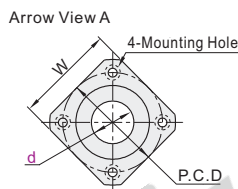
Square Flange OFZ32 OGA21
