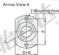
Compact Flange OFZ62 OGA41
