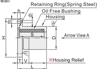
Compact Flange OFZ62 OGA41
