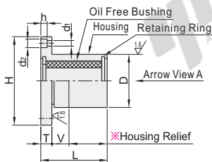
Round Flange OFZ02 OGA01
