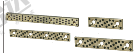
OBG02 (Plate Thickness 5mm)
