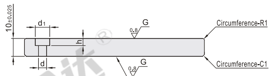
OBG12 (Plate Thickness 10mm)
