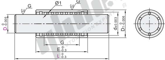
Holistic Type Bushing
