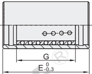
Holistic Type Bushing
