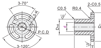
Slotted Holes LJP91
