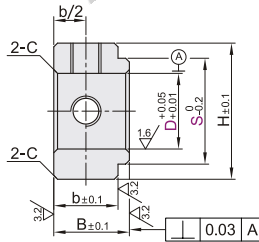
Short Shoulder FBC01/02/06/21/22
