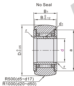
Crowned Type BPW05
