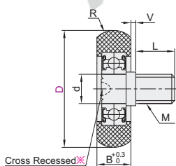
Threaded Stud BKR51 BKR52
