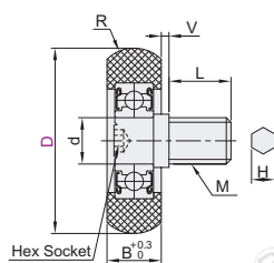
Threaded Stud Hex Socket BKR62
