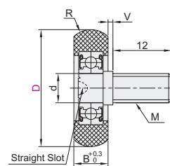
Long Threaded Stud BKR72
